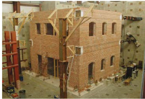
Full-scale testing of unreinforced masonry building.
