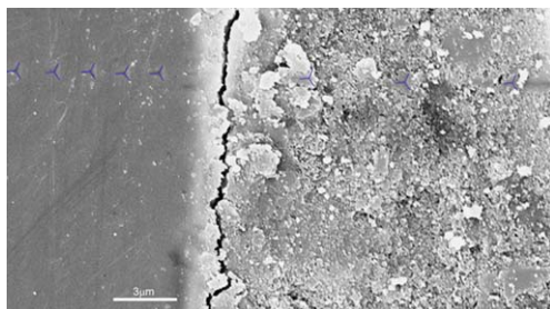
Nanoindentations in a nano-engineered, fiber-reinforced, ultra-high performance cementitious material.
