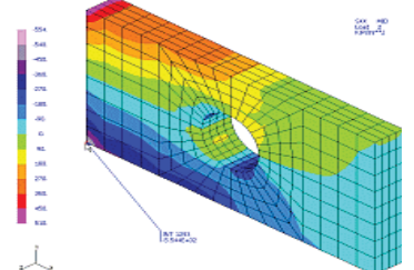
3D finite element modeling and simulation using GT STRUDL software.
